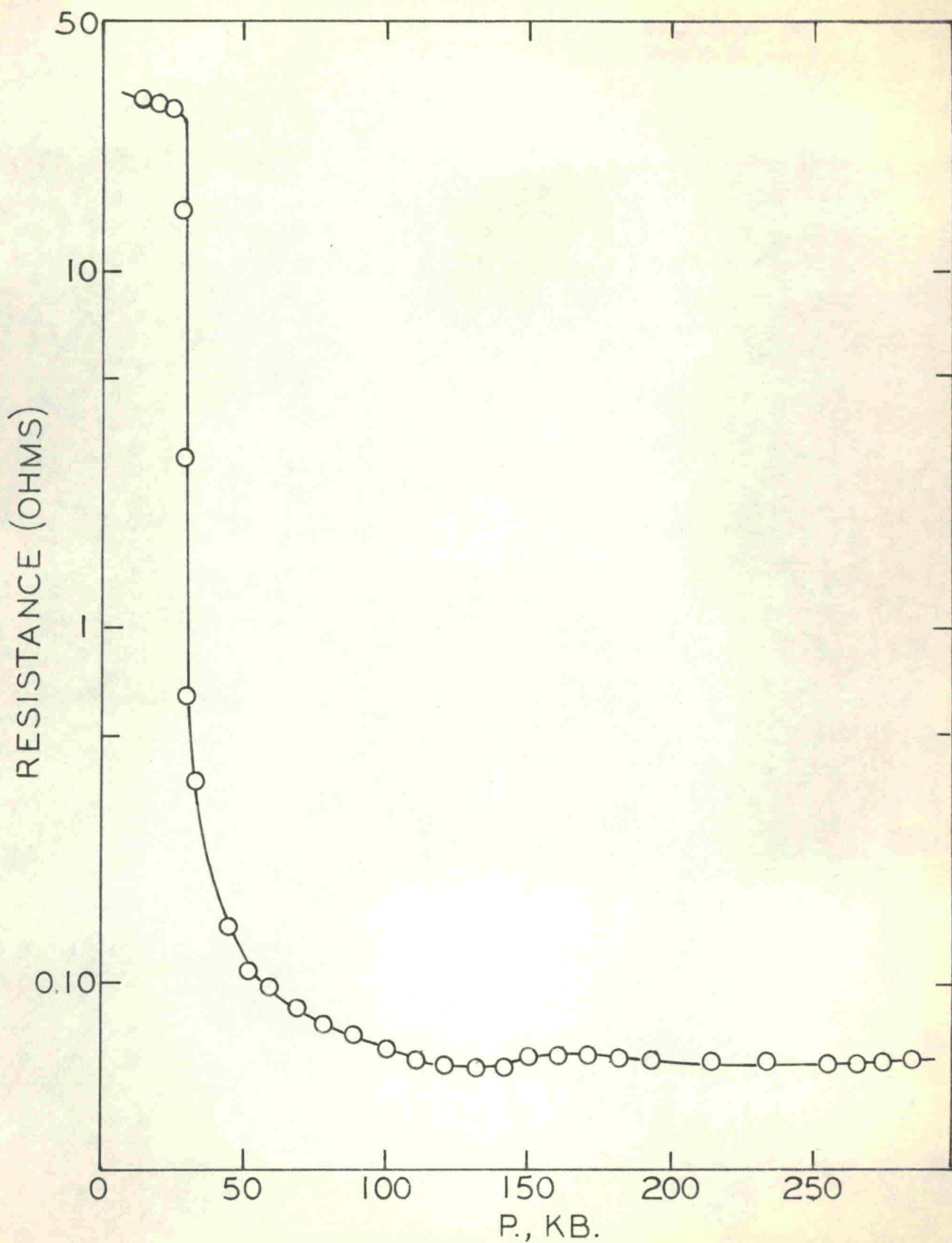
FIG.1 RESISTANCE VS. PRESSURE FOR CdSe
